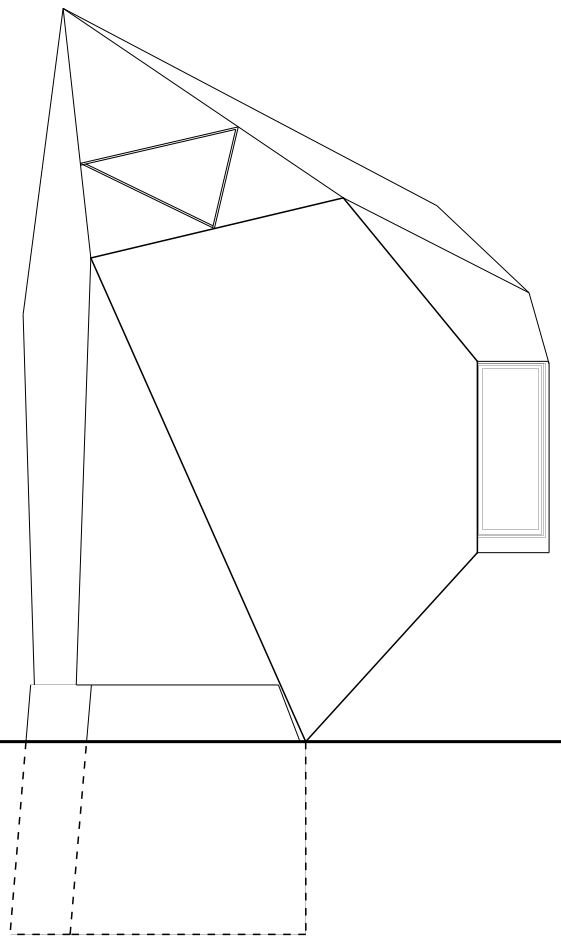
South elevation
